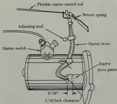
FIGURE 5-10. Starter lever controls and adjustment.
